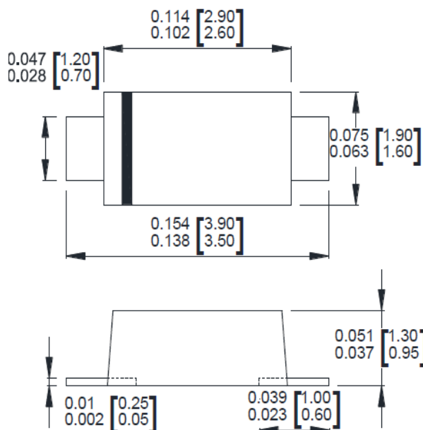
SOD-123FL
